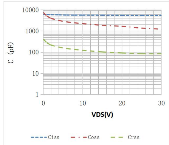
Fig.2 Capacitance Characteristics
